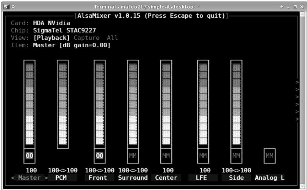
FIGURE 15.6 – alsamixer
