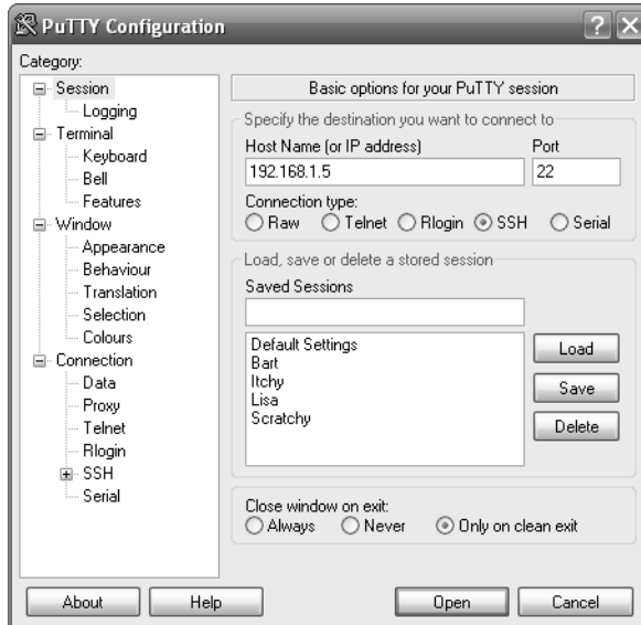
FIGURE 23.19 – PuTTY
