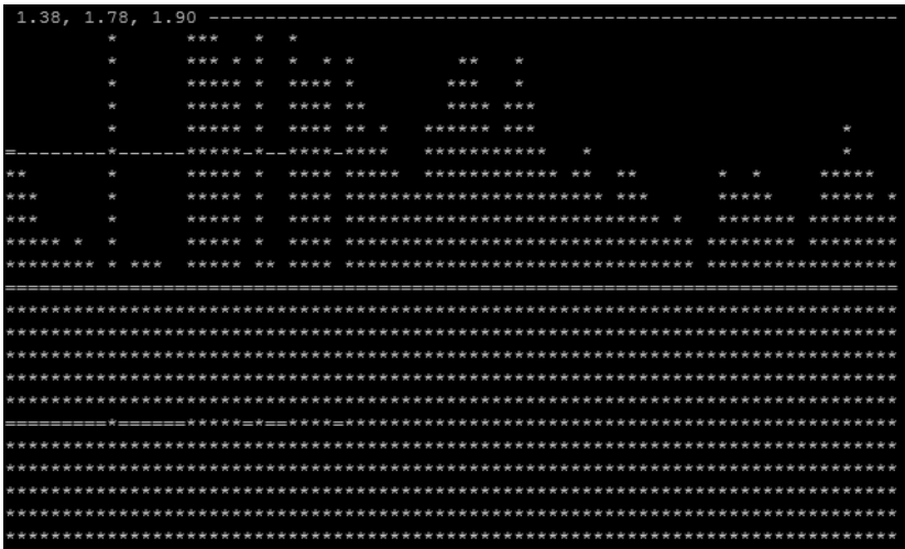
FIGURE 19.1 – Charge processeur
